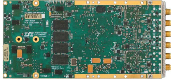
Figure 5. XU-AWG bottom side
